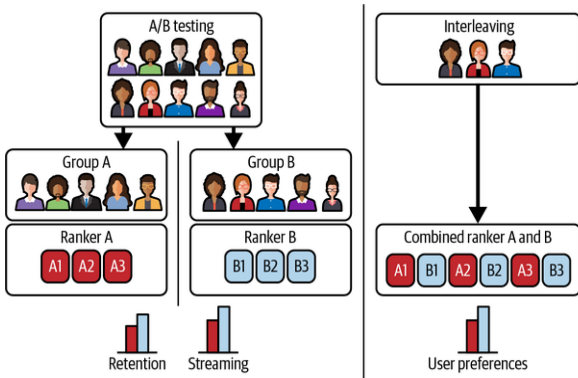
Figure 9-6. An illustration of interleaving versus A/B testing. Source: Adapted from an image by Parks et al.
