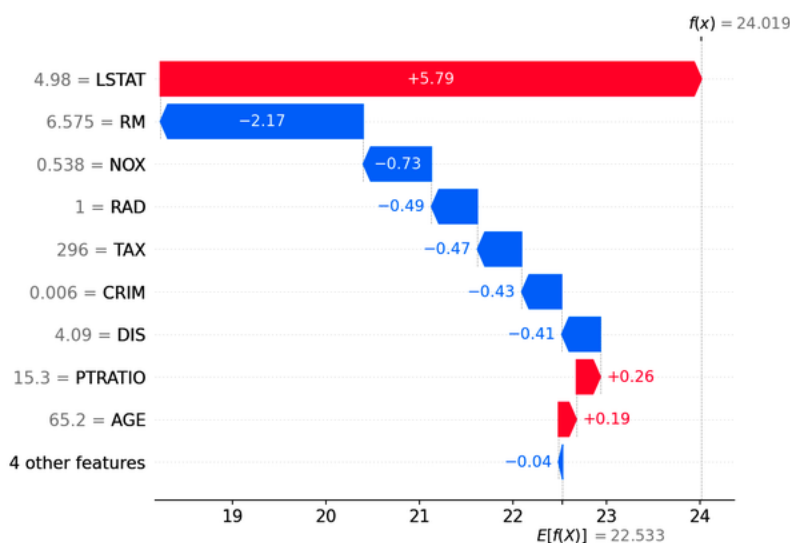
Figure 5-8. How much each feature contributes to a model's single prediction, measured by SHAP. The value LSTAT = 4.98 contributes the most to this specific prediction. Source: Scott Lundberg 19
