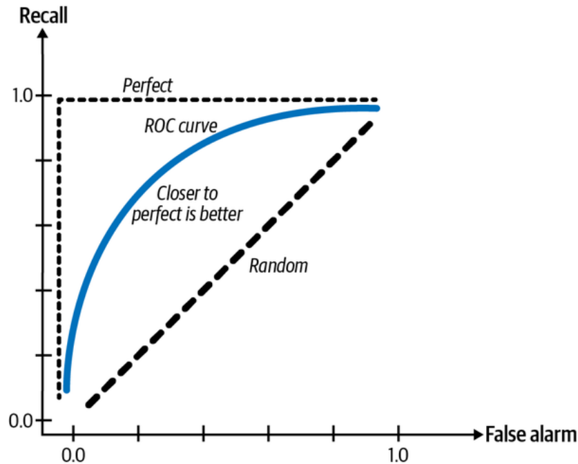
Figure 4-9. ROC curve
